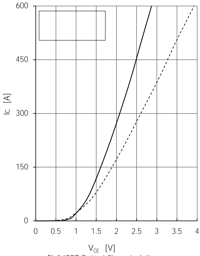
Fig1.IGBT Output Characteristics
