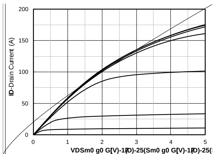
Figure 1. Output Characteristics
