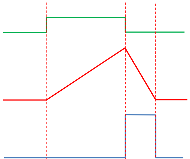
Figure A. Unclamped Inductive Switching (UIS) Test Circuit & Waveform
